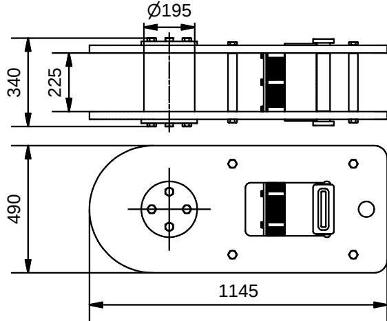
Anchor (1:20)
